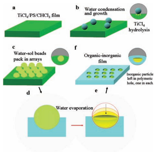
Figure 3. Scheme of formation of the highly ordered asymmetrical inorganic particle/polymer composite films by BFs method.
